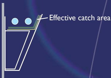
Luralite Plus glueboard positioning
